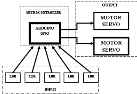
Gambar 1. Diagram Blok Solar Tracker
