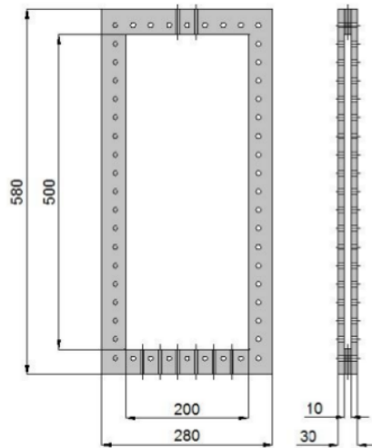
Gambar 1. Dimensi Helle Shaw Cell
