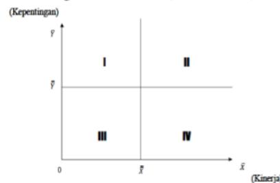
Gambar 3.1 . Diagram Kartesius Importance and Performance Analysis (IPA)
