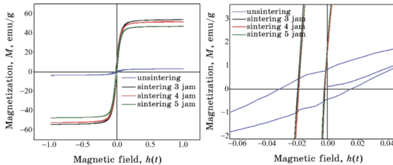
Fig. 3. VSM test results on manganese–zinc ferrite ( Mn_{0.8}Zn_{0.2}Fe_2O_4 ) unsintered and 3, 4, and 5 hours holding time sintered graphic.
