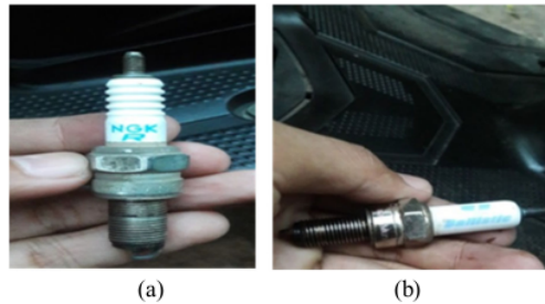
Gambar 2. Busi (a) standar, (b) iridium
