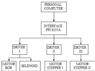
Gambar 8 Diagram Blok Alat
