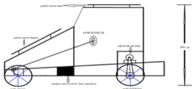
Gambar 5. mobil sel surya tampak samping
