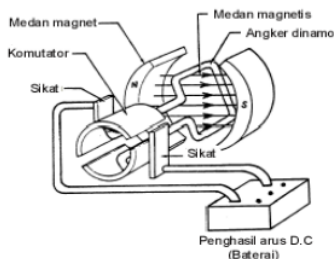
Gambar 1. Motor D.C magnet permanen
