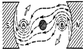
Gambar 2. Reaksi garis fluks.
