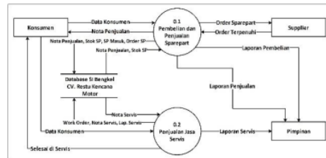
Gambar 3.5 DFD Level 0
