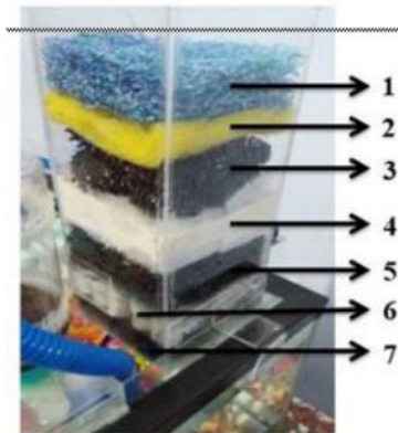
Gambar 12. Filter Hybrid
