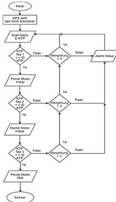
Gambar 8. Flowchat Sistem
