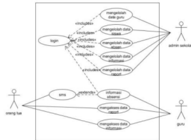
Gambar 3.2 Use Case
