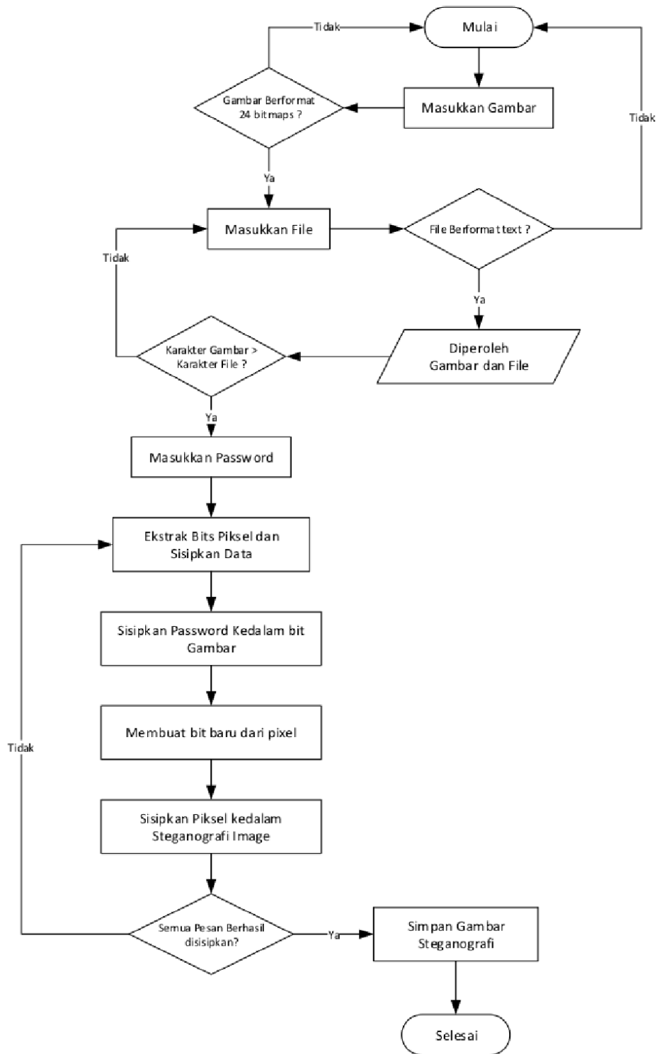
Gambar 4 : Diagram alir Decode
