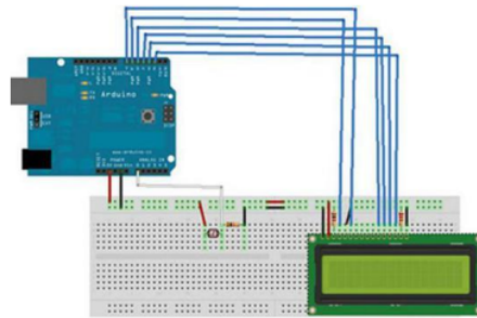
Gambar 8. Wiring diagram
