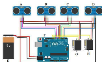
Gambar 7 perancangan hardware
