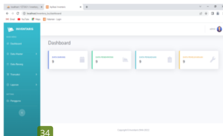
Gambar 4.2 halaman dashboard
