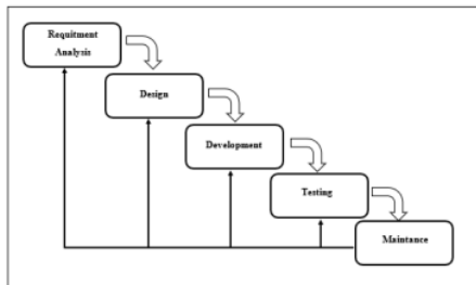
Gambar 3.2 Metode Waterfal
