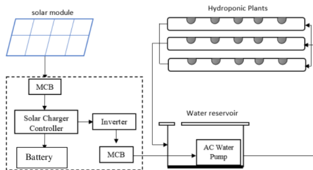
Figure 3. Solar Hydroponic Plant Series Using AC Motor
