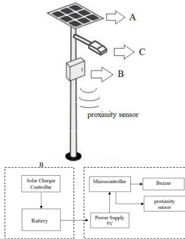
Figure 1. PJUTS with Security System
