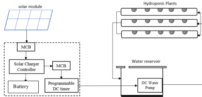
Figure 2. Solar Hydroponic Plant Series Using DC Motor
