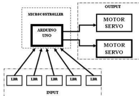
Gambar 1. Diagram Blok Solar Tracker
