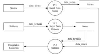
Gambar 7. DFD Level 1
