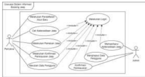
Gambar 3: Usecase Diagram
